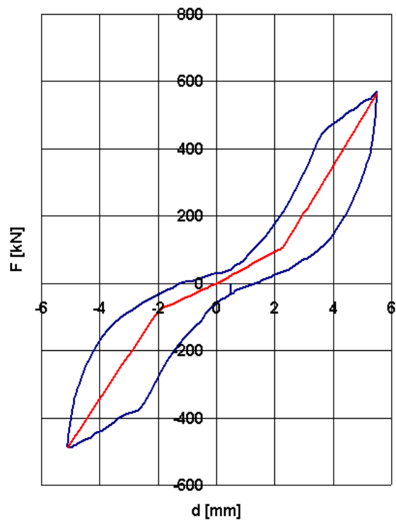
Fig. 3.6. Force- distortion hysteresis diagram
