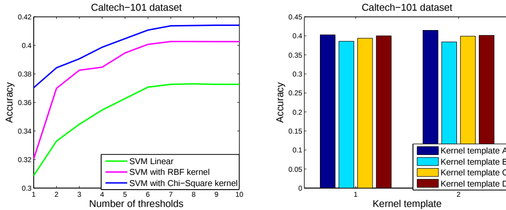
FIG. 4. The influence of parameters on the system performance: (1) the variation of the thresholds number and the SVM kernel and (2) the performance of various template functions.
