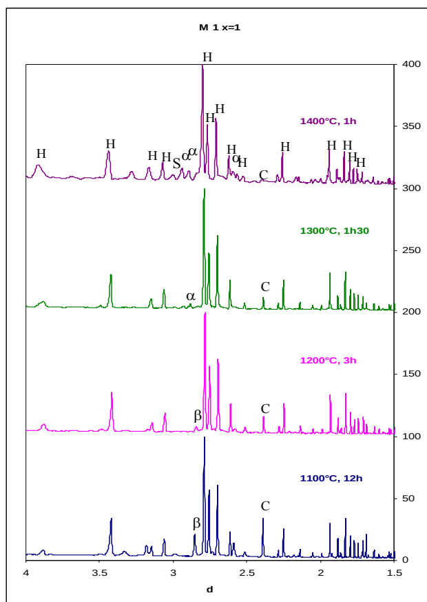
Fig. 2: X-Ray diffraction patterns of M1 with x=1 after heating at different temperatures; H- hydroxyapatite, S-silicocarnotite, \alpha - \alpha tri calcium phosphate; \beta - \beta tri calcium phosphate; C-calcium oxide (lime)
