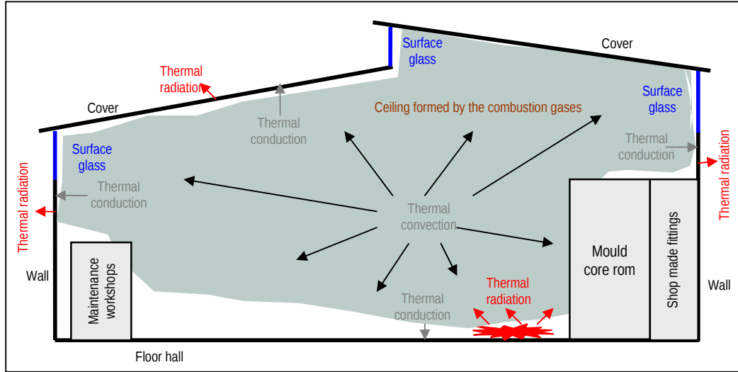
Fig. 4 Heat transfer inside the foundry hall
