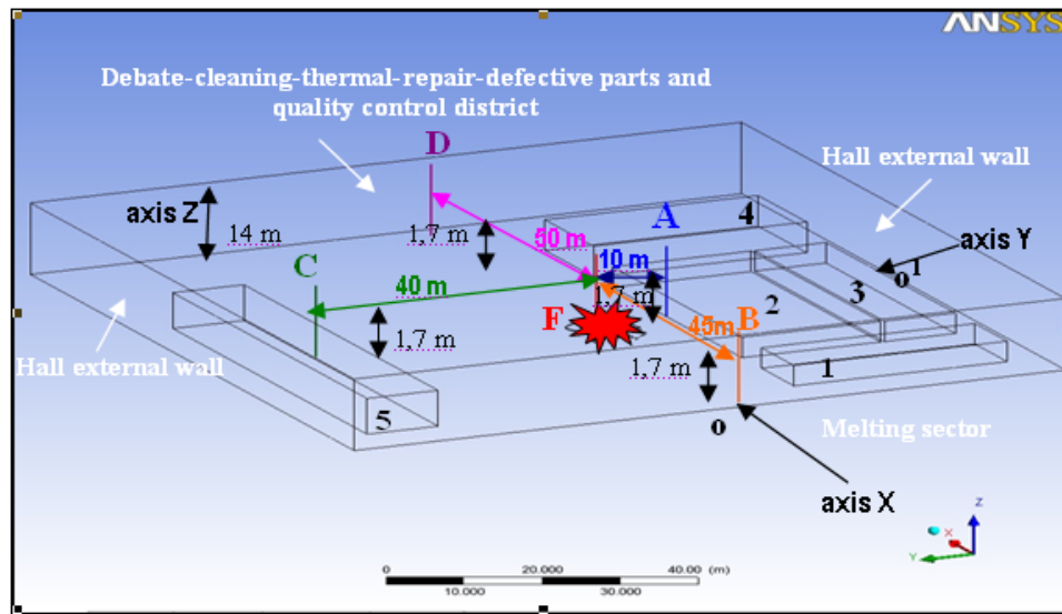
Fig. 6. Points where temperature measurements were made: 1- District of moulding mixture preparation and core training, 2- District of cores manufacture (drying, assembly and painting cores), 3- Shop fittings manufacturing cores, 4- Storage models, 5- Maintenance Workshops (mechanical, electrical, mechanical processing etc.). 4.5. Input
