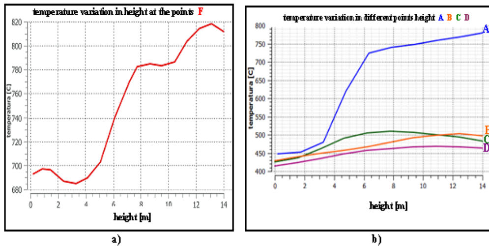
Fig.11 The temperature variation at the end of simulation ( M = 600 s) the hall height (Z axis): a) above the focus (point "F"), b) above the points "A", "B", "C" and "D".
