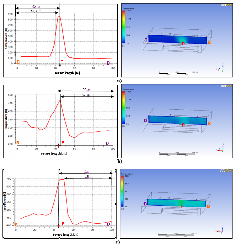
Fig. 7 Temperature variation along the length of the casting sector (X axis) at 1.7 m height at the moments: a) M = 60 s, b) M = 300 s, c) M = 600 s
