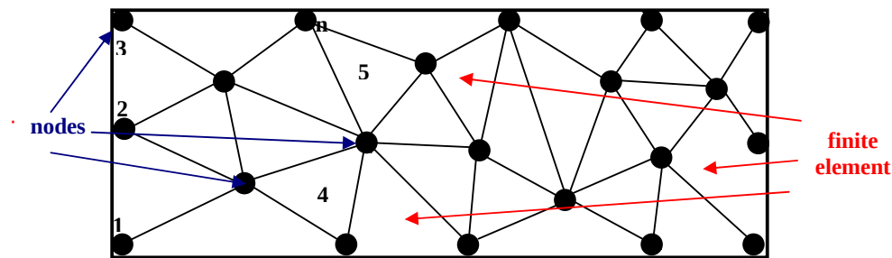
Fig. 5 Meshing domain
