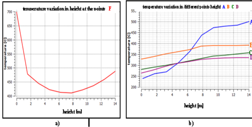
Fig.10 The temperature variation at M = 300 s the hall height (Z axis): a) the point "F" (above focus), b) the points "A", "B", "C" and "D".
