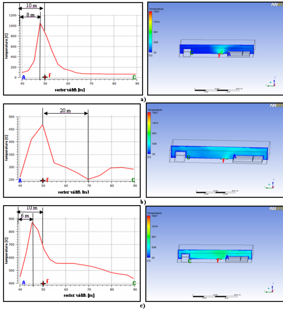
Fig. 8. The temperature variation across the width of the casting sector (Y axis) at 1.7 m height at moments: a) M = 60 s; b) M = 300 s; c) M = 600 s.
